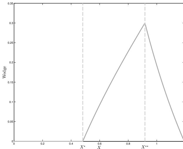
Figure 2: Labor wedge as function of X .
