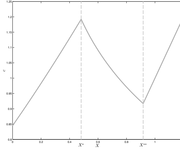
Figure 3: Consumption as function of X .
