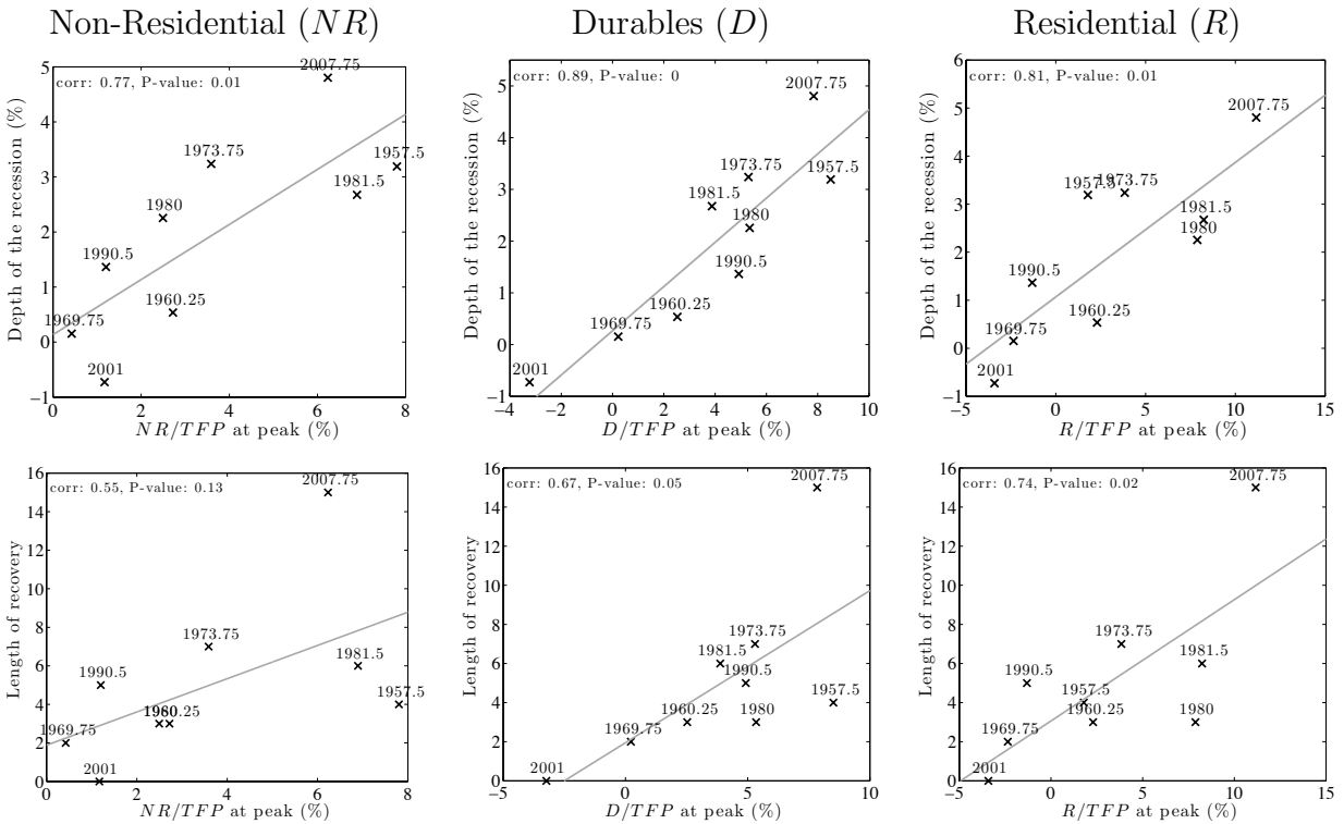
Figure 1: Depth of recession and length of recovery vs. cumulated investment
